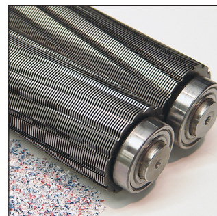
Dahle High Security cutting cylinders reduce a sheet of paper to over 15,500 pieces.
